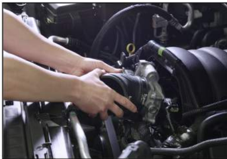
14. Install INLET/DUCT onto throttle body. Leave all connections loose.
